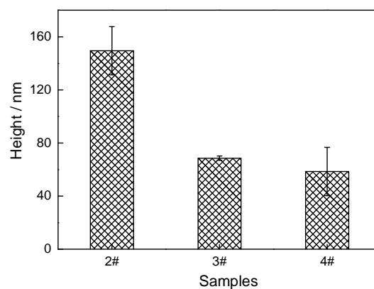
图7 不同 DLC 处理样品与 PET 基体之间的高度差 Fig.7 Height between different samples with DLC deposited and PET substrate
